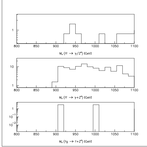
Figure 3.5: Histograms for the contributing backgrounds for the process X \rightarrow Z^0 \gamma \rightarrow \bar{l} l \gamma for m_X \sim 1000 GeV, after preselection cuts.
